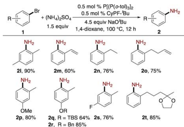
Scheme 4. Scope of Palladium-Catalyzed Amination of Ortho -Substituted Aryl Bromides with Ammonium Sulfate a
